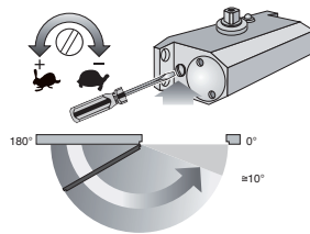
Closing speed adjustment (180°-10°).
