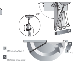
Adjustment of final latch angle (10°-0°).
