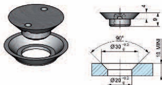
50 stainless steel caps with rings
