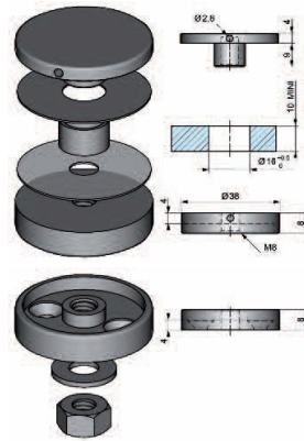
Top and bottom threaded top flat head set for 33 mm Ø tube
