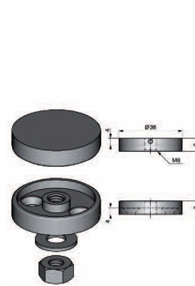
Top and bottom top glued head set for 33 mm Ø tube
