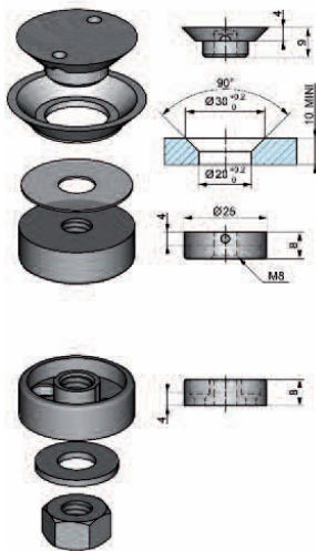
Top and bottom threaded top countersunk head set for 21 mm Ø tube
