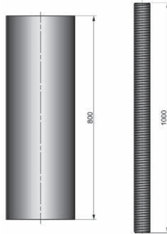
33 mm Ø 300 mm long stainless steel tube with M8 threaded rod
