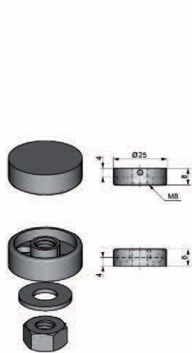
Top and bottom top glued head set for 21 mm Ø tube
