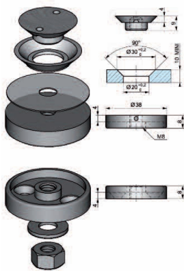
Top and bottom threaded top countersunk head set for 33 mm Ø tube
