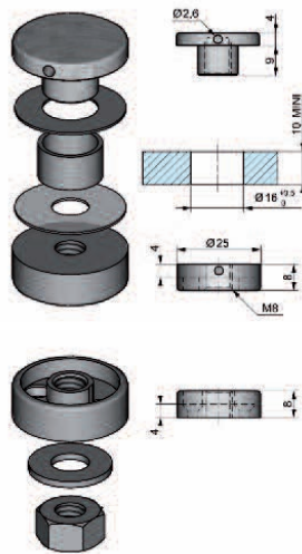
Top and bottom threaded top flat head set for 21 mm Ø tube
