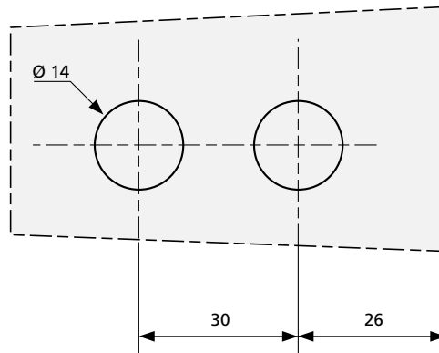
Notch 3062E 135° - Fixed Panel
