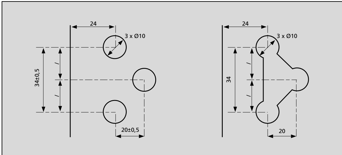
Notch 648/3 Incorporates 648/3 and 648/1
