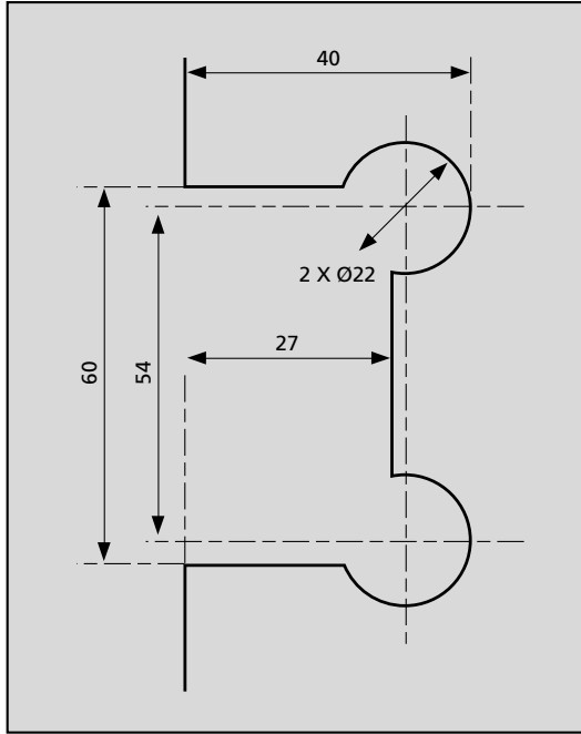
Notch 648/7 includes 648/7 and 648/6
